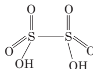
Dithionic acid ( \text{H}_2\text{S}_2\text{O}_6 )
